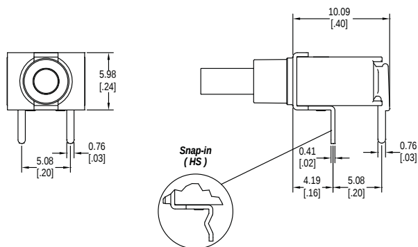
H (HS - Snap In) = Horizontal mount, right angle PC pins, SPST
